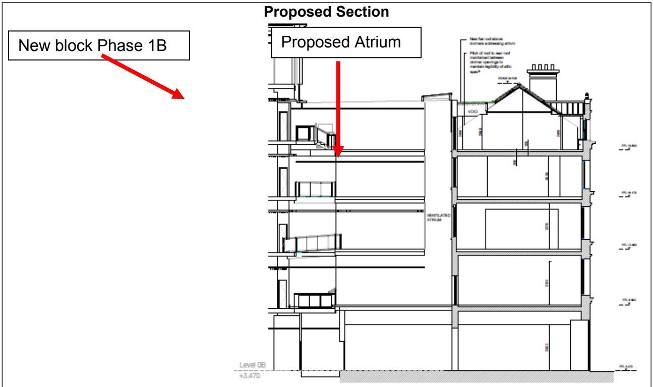
41-51 Royal Avenue - Proposed Section BB
